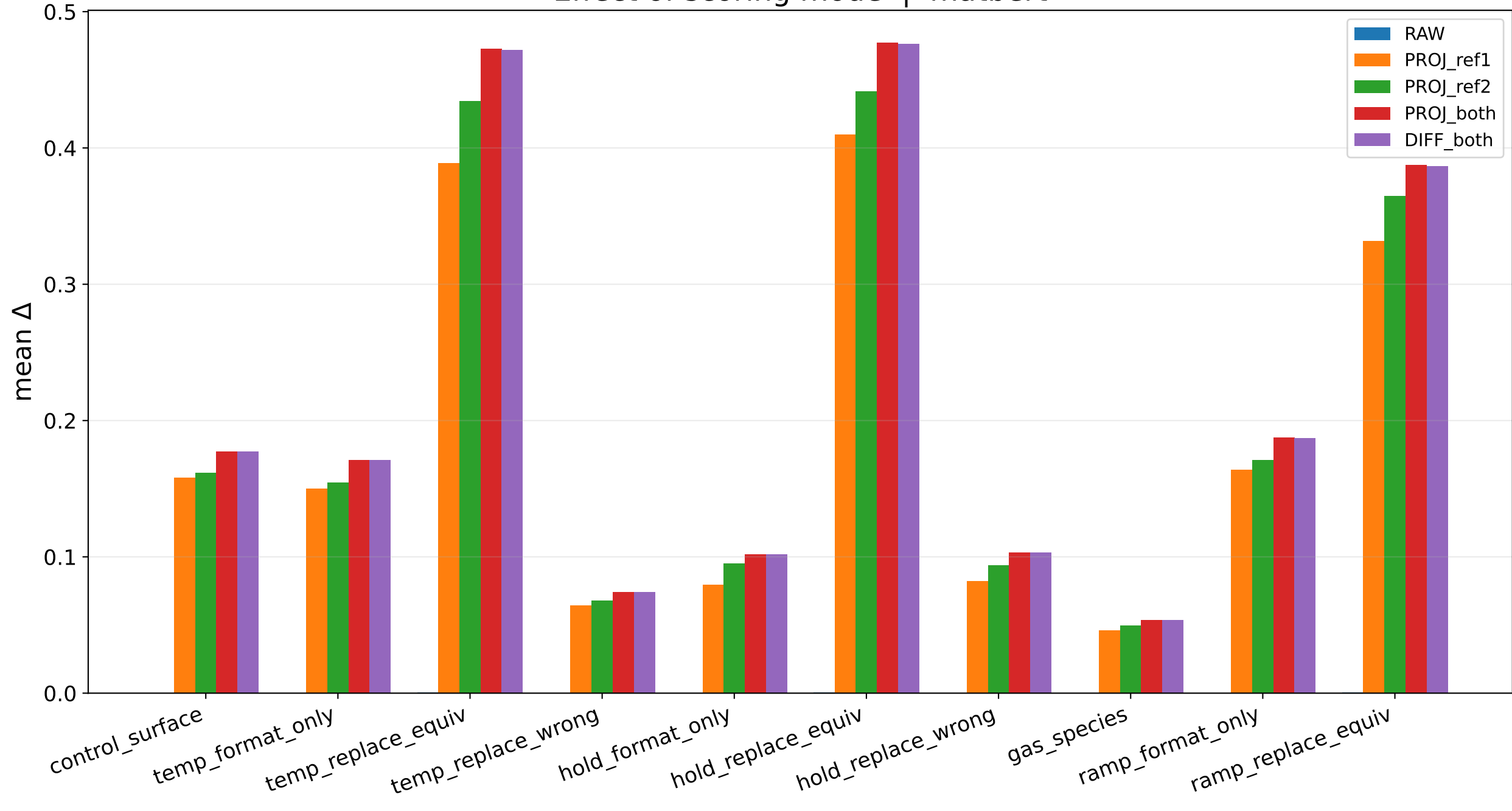
Effect of scoring mode | matbert
